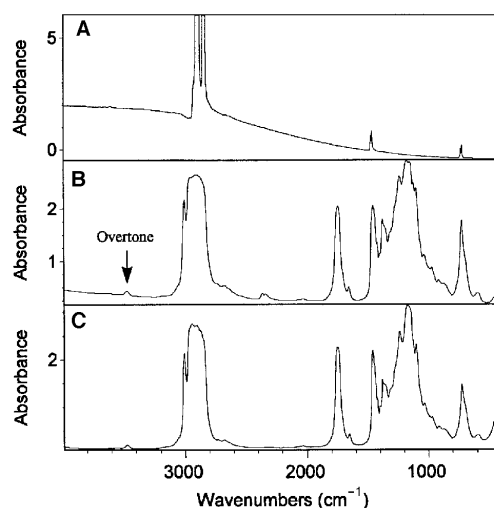
FIG. 2. (A) Spectrum of a 100\text{-}\mu\text{m} polyethylene (PE) IR card, (B) spectrum of a card loaded with canola oil, and (C) spectrum of canola oil in a 100\text{-}\mu\text{m} KCl flow cell.
