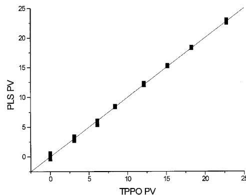
FIG. 6. Partial-least-squares (PLS) calibration plot for the 3M card method. PLS-predicted PV is plotted vs. calculated PV (based on TPPO concentration) for the calibration standards. The linear regression equation for the plot is y = 0.002 + 0.999x ; r = 0.999 , \text{SD} = 0.26 . For abbreviations see Figure 4.
